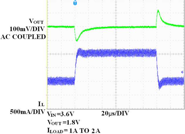
Load Step
