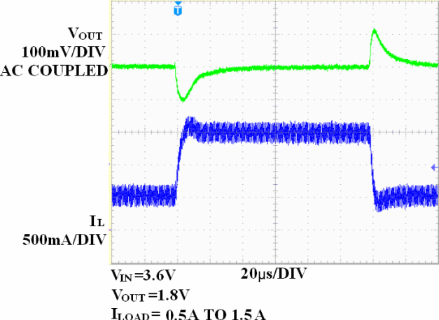
Load Step
