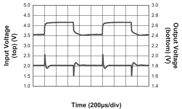
Line Transient Response ( V_{OUT} = 1.8V ; 1.5A Load)
