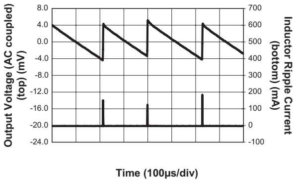
Light Load Switching Waveform (PFM Mode; V_{IN} = 3.6V ; V_{OUT} = 1.8V ; 1mA Load)
